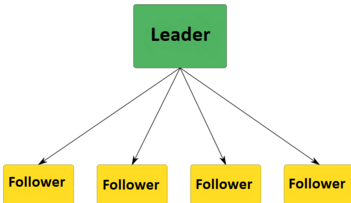
Figure 4.1: Leader/FollowerModel
