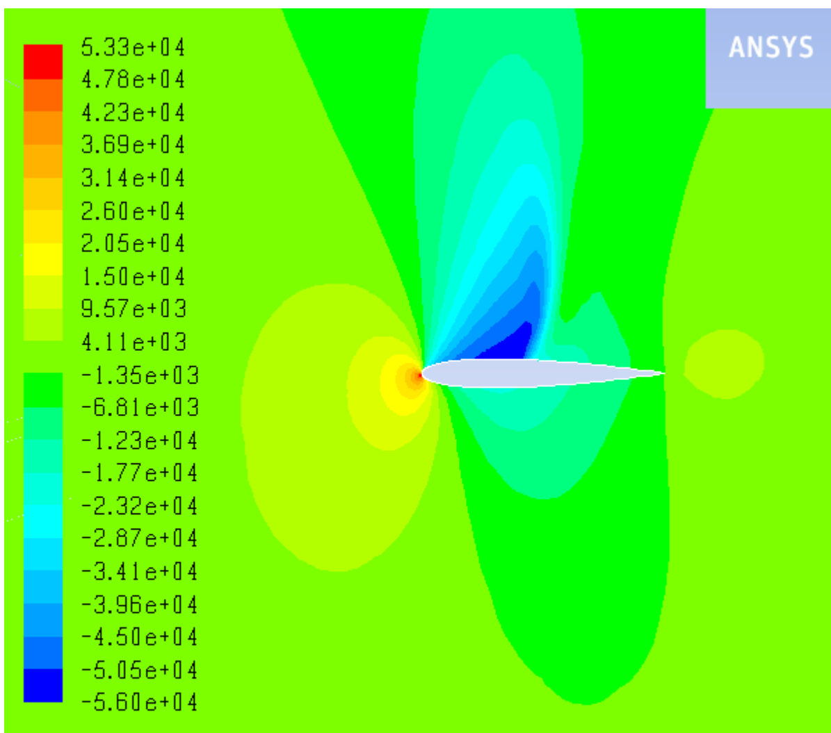
Contours of Static Pressure (pascal) ANSYS Fluent (2d, dp, pbns, S-A)
